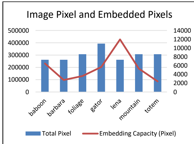
Fig 10: Compare between Image Pixels and Embedded Pixels
