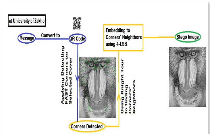
Fig 7: The proposed steganography model's embedding stages.
