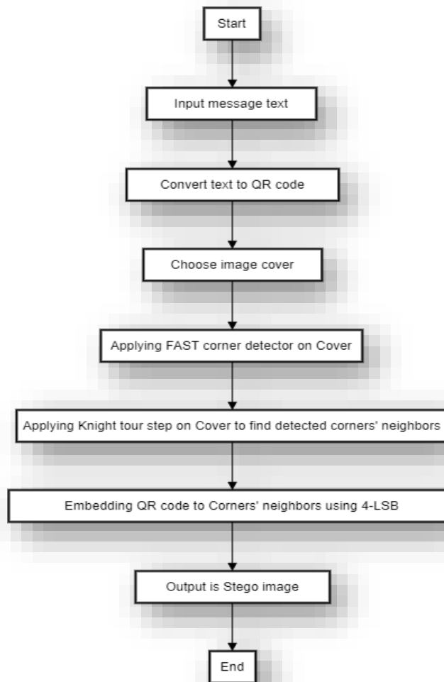
Fig 8: Embedding stage flowchart
