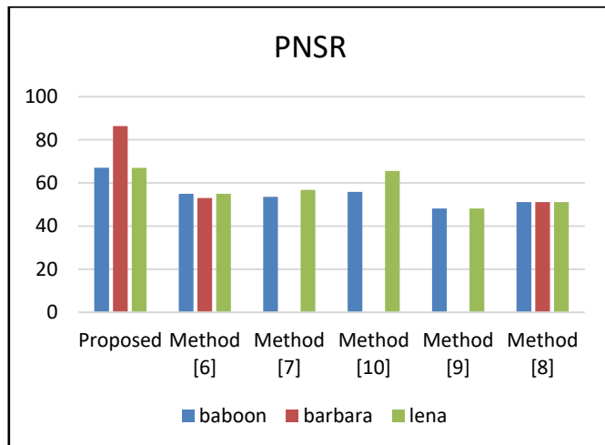
Fig 12: PSNR Comparative
