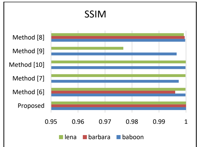
Fig 13: SSIM Comparative
