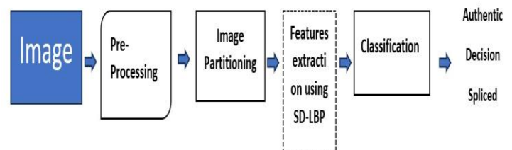
Figure. 1. Block diagram of the proposed algorithm
