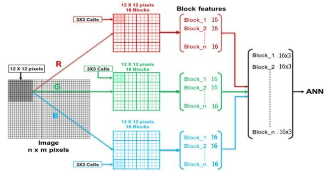
Figure 6. Feature vectors extraction.
