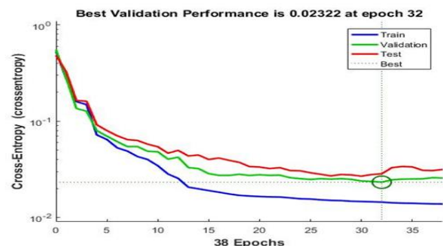
Figure 9. Training, Validation and Testing performance at epoch 32 shows the high validation performance (0.02322).
