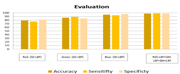
Figure 7. Experimental results from tampered images detection CASIA TIDE V 2.0.
