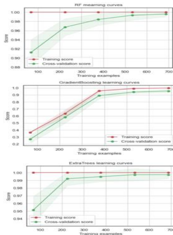
Figure 7(a)-(e): Learning curve of the various models
