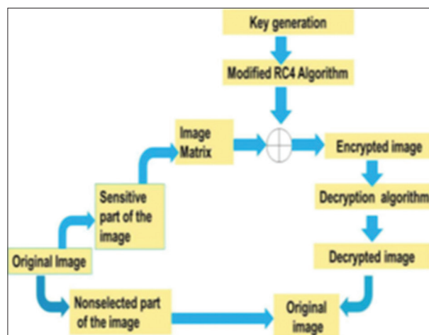
Fig 1: Methodology of RC4 algorithm.
