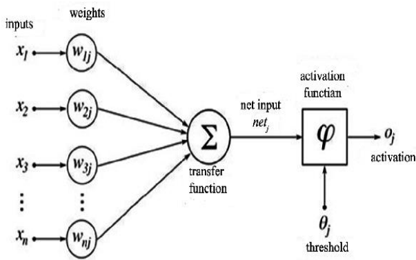
Fig 2: Artificial Neural Networks Model [3]
