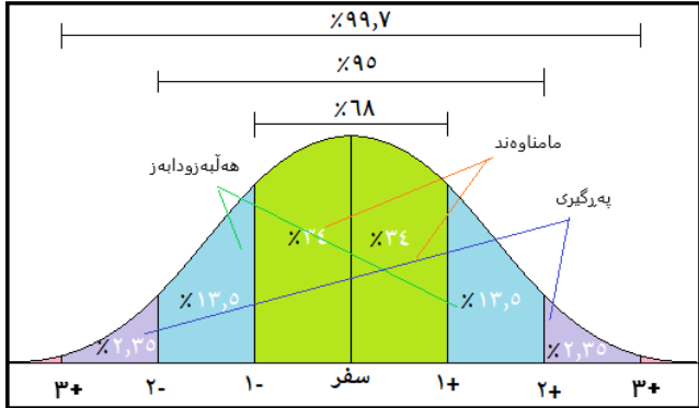
سەرچاۋە: نامادەكرائو پىشت بەست بە Dietmar Dommengat, An Introduction to Statistical Analysis in Climate Research, Figure 3.9, Normal Distribution, 2015, p29
